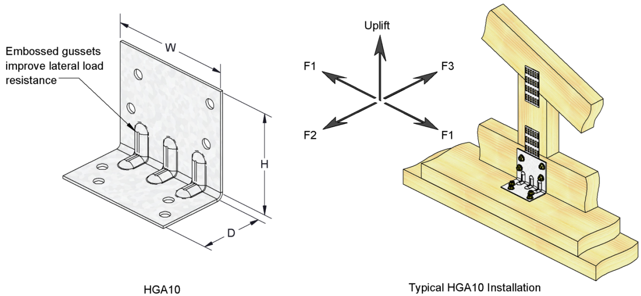
FIGURE 6—HGA HURRICANE GUSSET ANGLE
