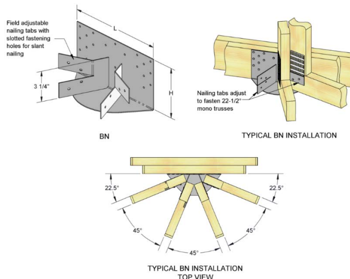
FIGURE 1—BN BREAKFAST NOOK HANGER
