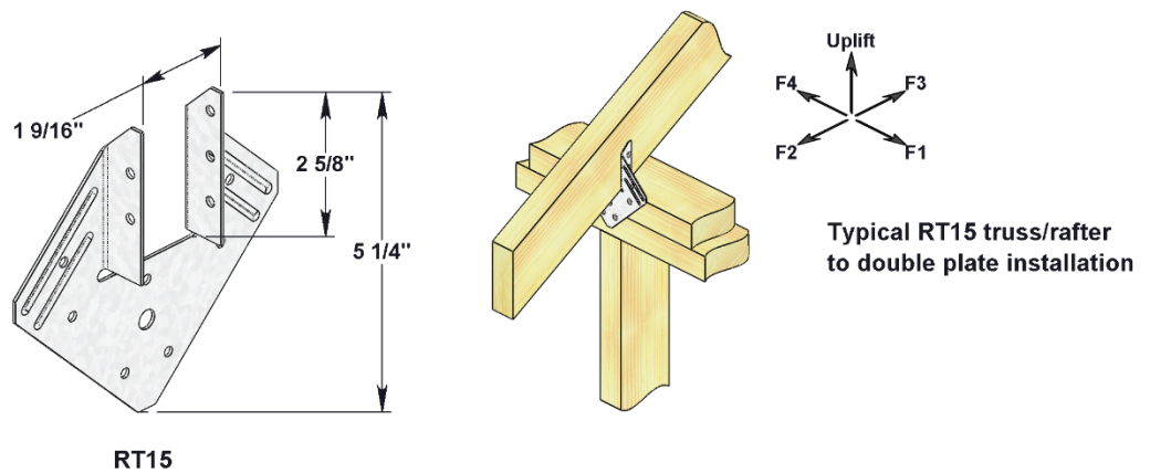
FIGURE 9—RT HURRICANE TIE (Continued)
